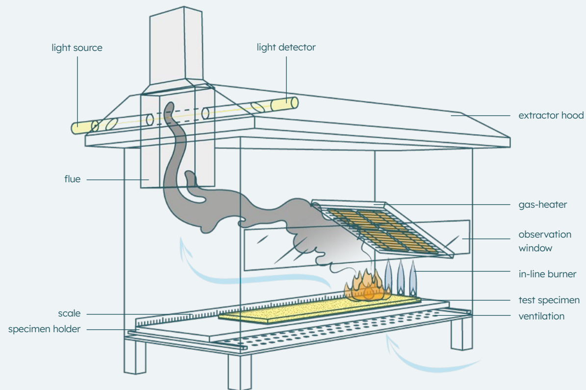
Fig. 64: testing reaction to fire
