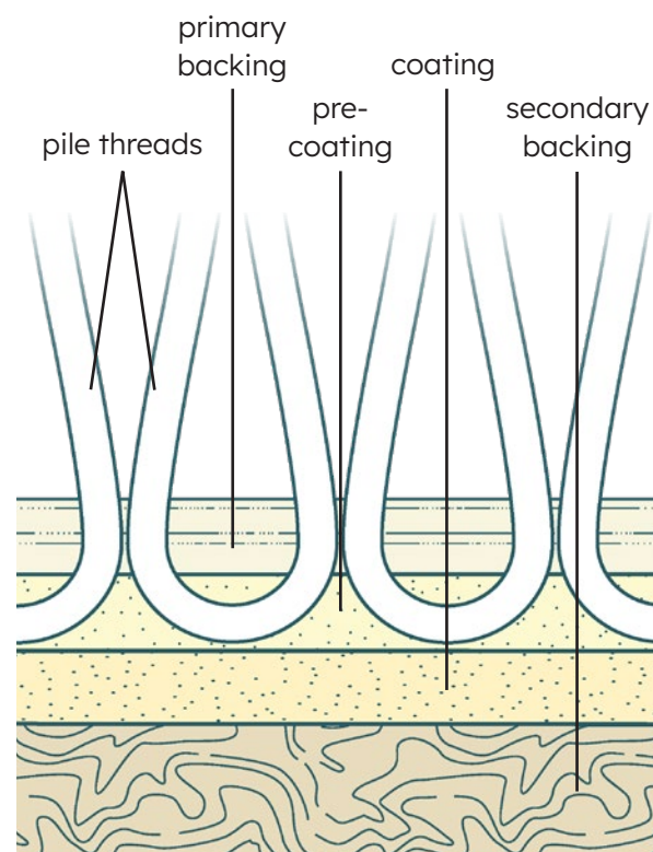
Fig. 11: layers of tufted carpet
