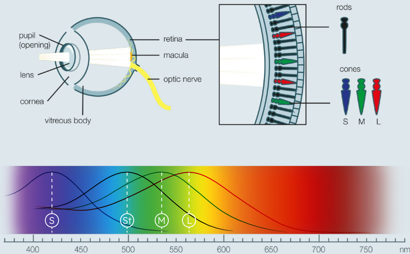
Fig. 8: the eye
