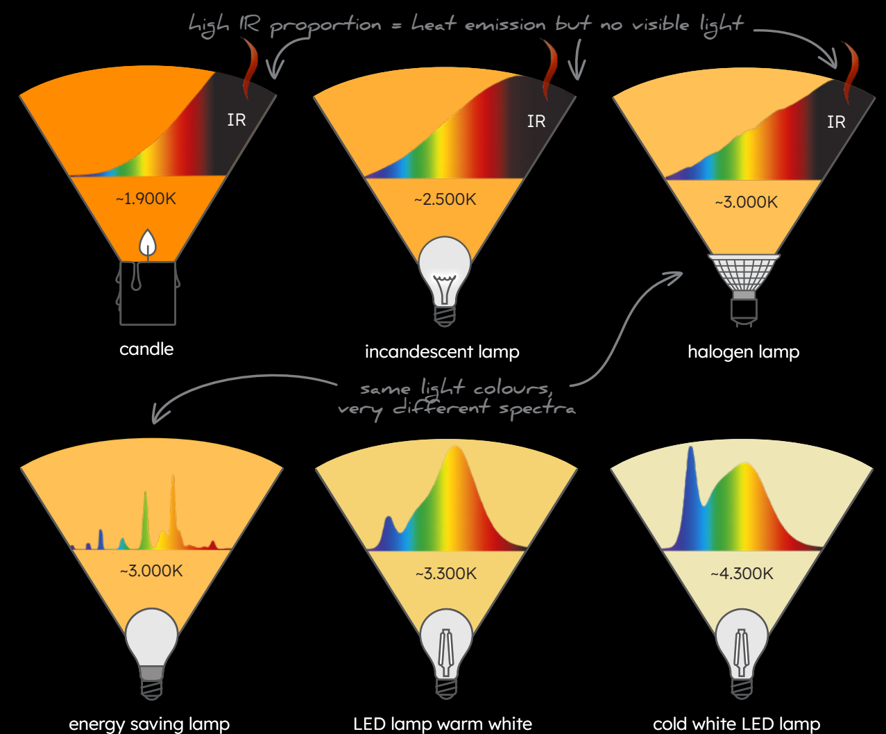
Fig. 5: light spectra of different light sources
