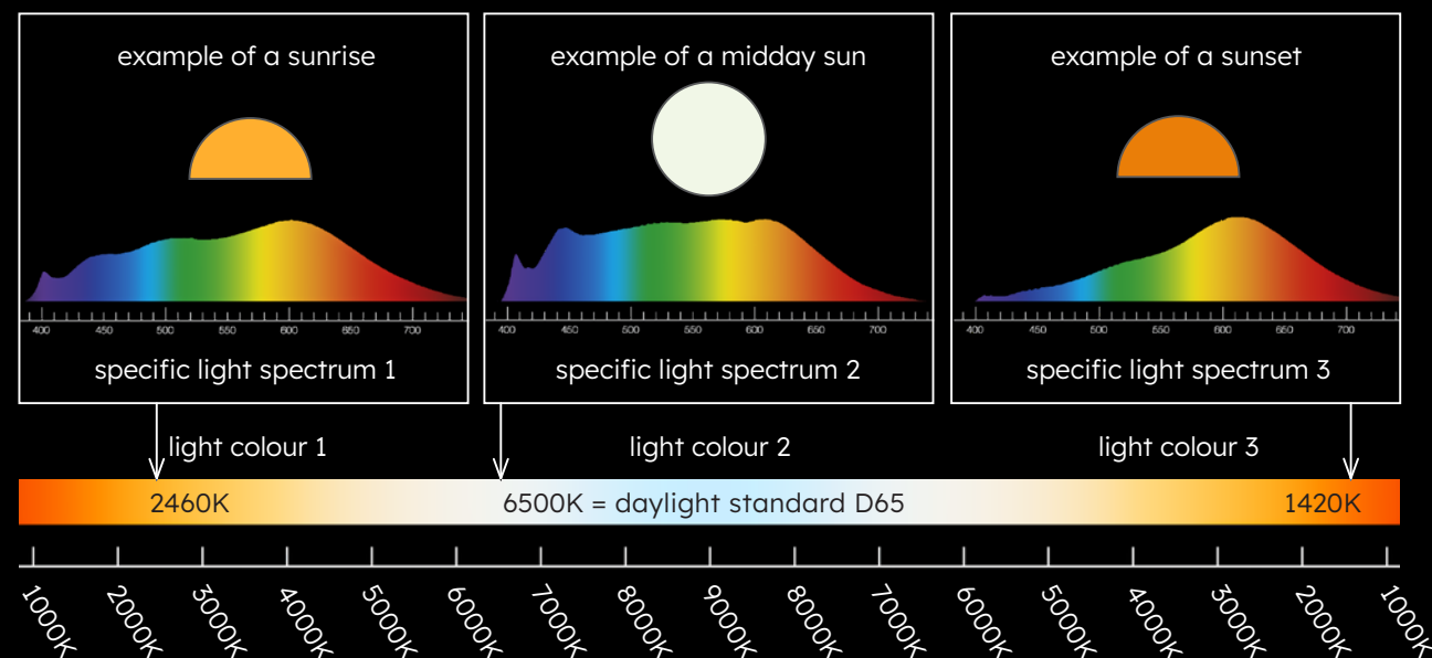
Fig. 4: time of day - light spectrum - light colour
