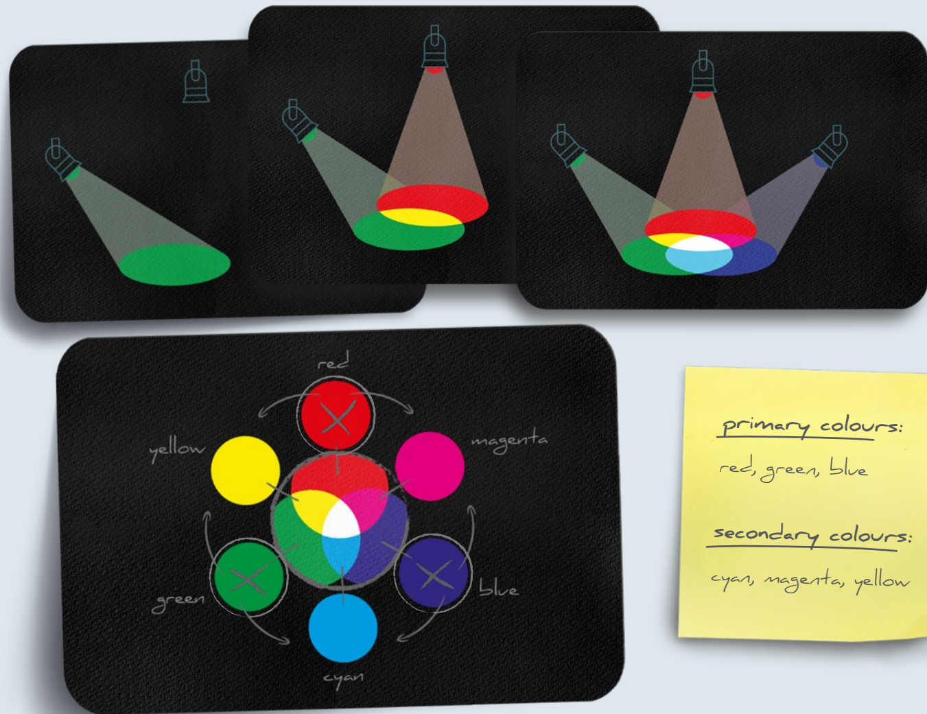
Fig. 18: light colours - additive mixing
